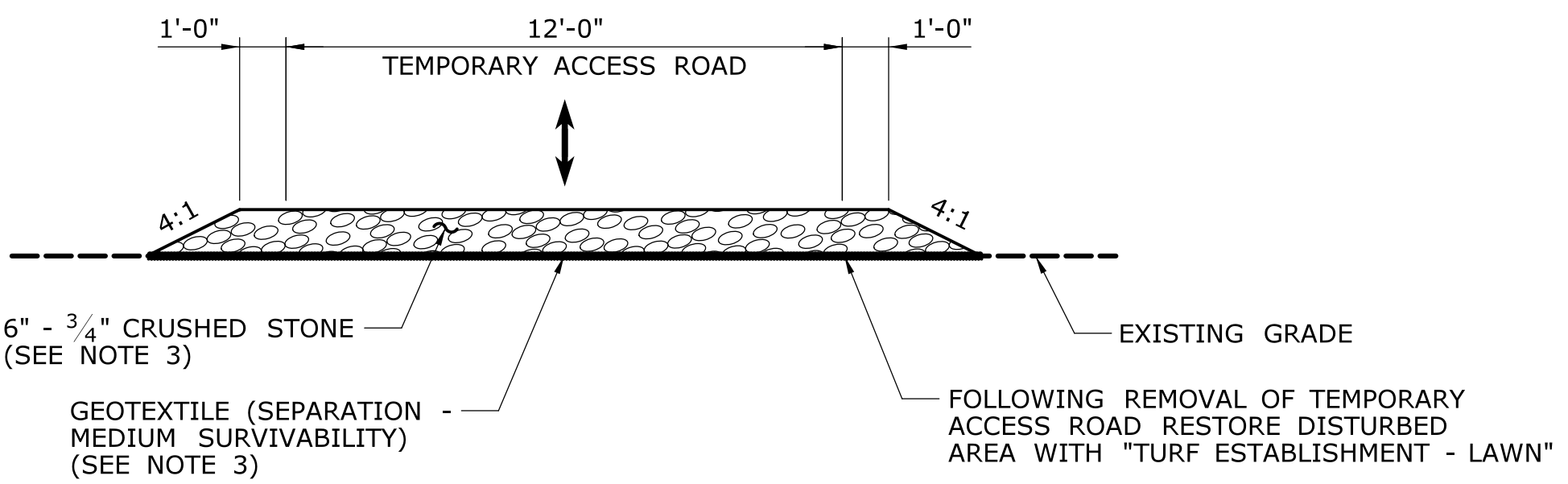
TEMPORARY ACCESS ROAD DETAIL NOT TO SCALE
